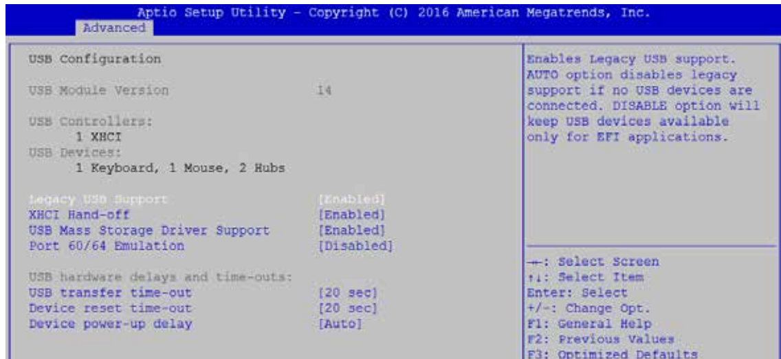
Figure 4 3-14: USB Settings
