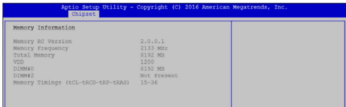
Figure 4-4-4: Memory Information
